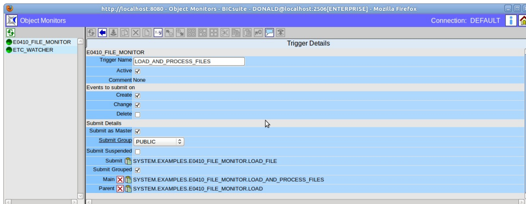
Abbildung 25.7: Object Monitoring Trigger Details
