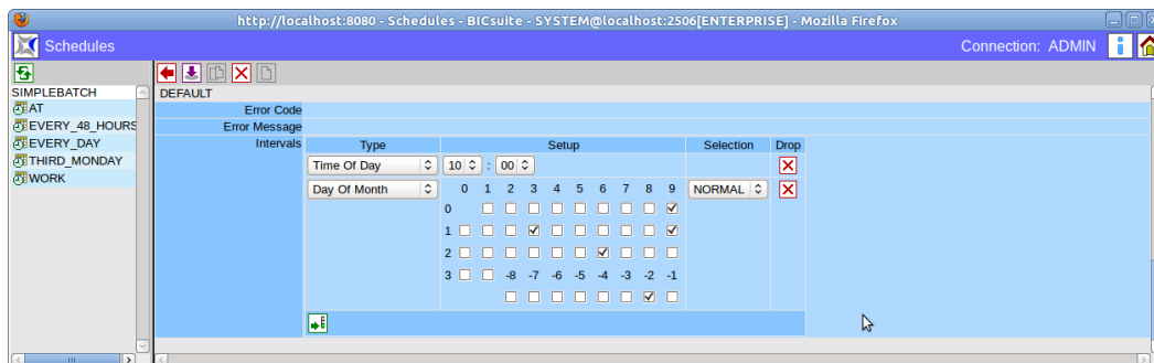
Abbildung 18.8: Day of Month Filter
