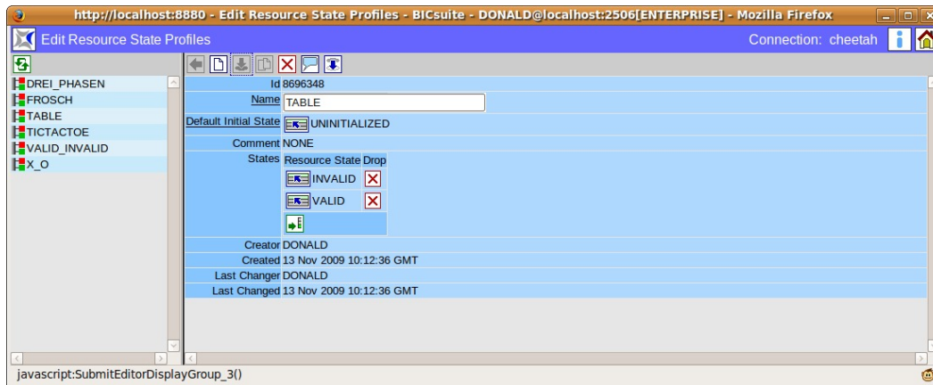
Abbildung 7.2: Resource State Profile Editor
