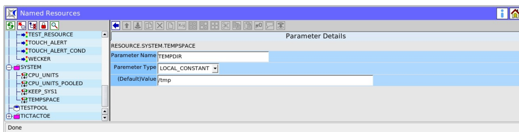
Abbildung 10.6: Named Resources; Parameter Details
