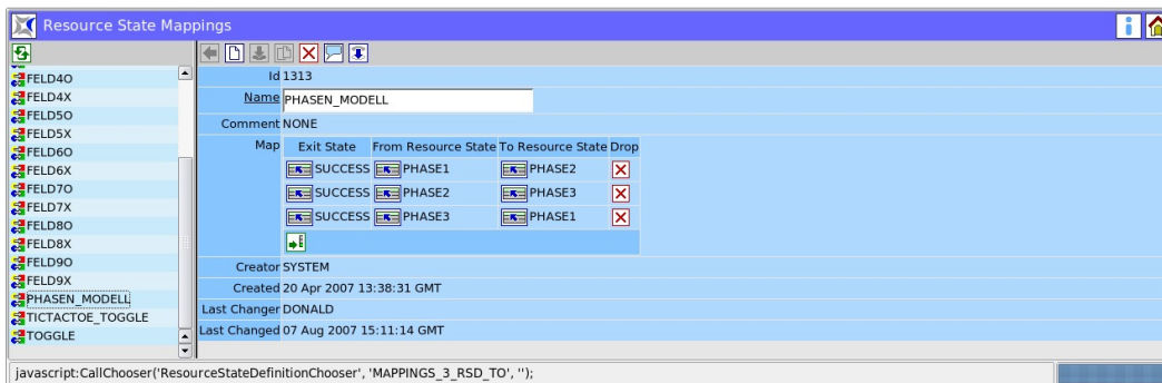
Abbildung 8.3: Resource State Mapping Editor
