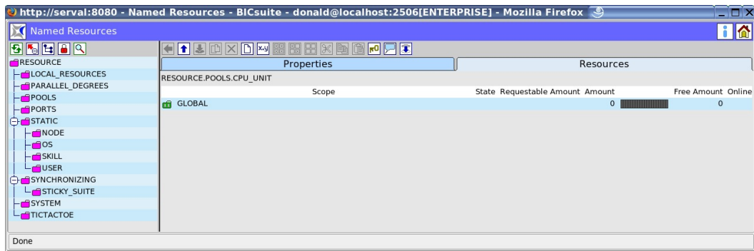
Abbildung 10.10: Named Resources; Pool Instanzen
