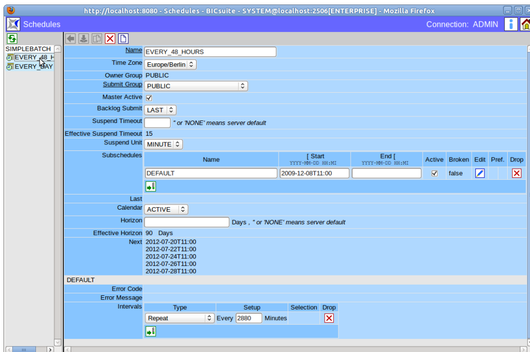
Abbildung 18.2: Time Scheduling Navigator
