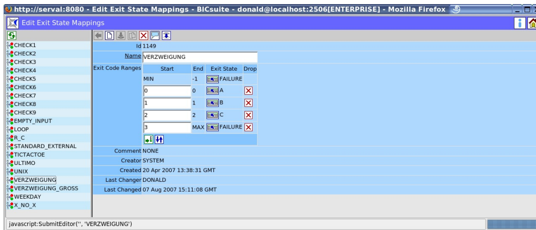
Abbildung 3.2: Exit State Mapping Editor
