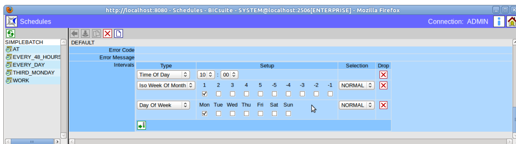
Abbildung 18.10: ISO Week of Month Filter
